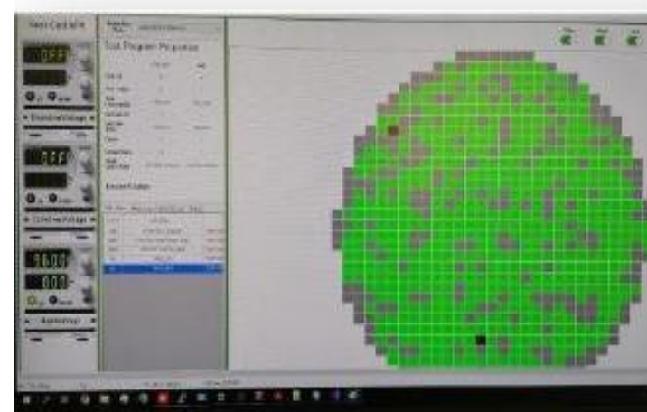
Software Platform
